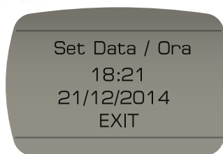
SETTINGS
