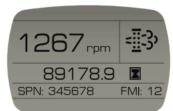
ENGINE ERROR
