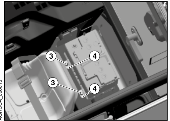
Low profile Cab version
